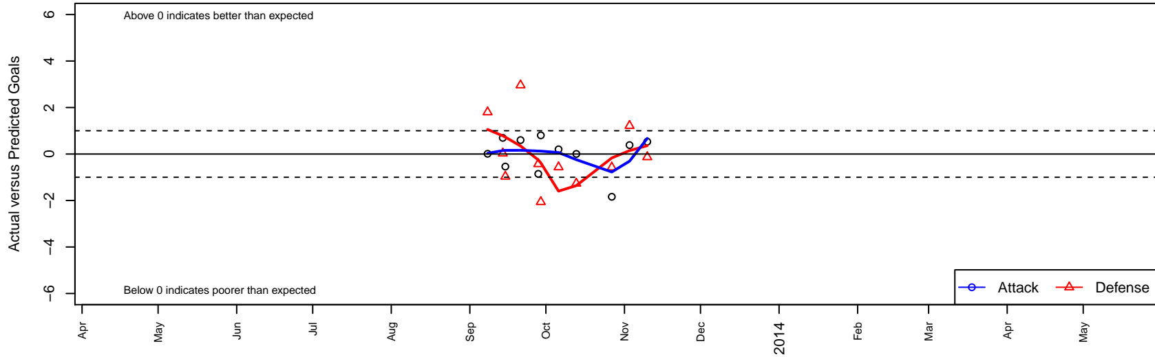
Legacy FC Dynasty B94 Dots are actual minus expected GF (blue circles) and GA (red triangles). Blue line is smoothed change in attack strength. Red is smoothed change in defense strength.
